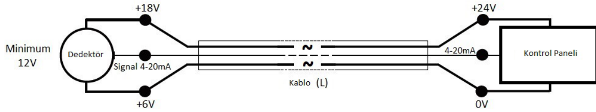
Diagram 7: Sahada kablolama
