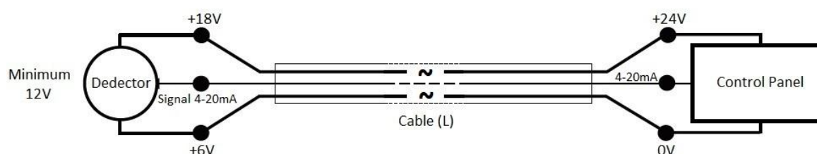
Diagram 5: Field cabling
