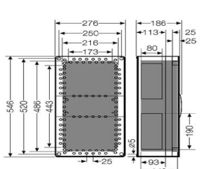
DP8 and DP32 Dimension
