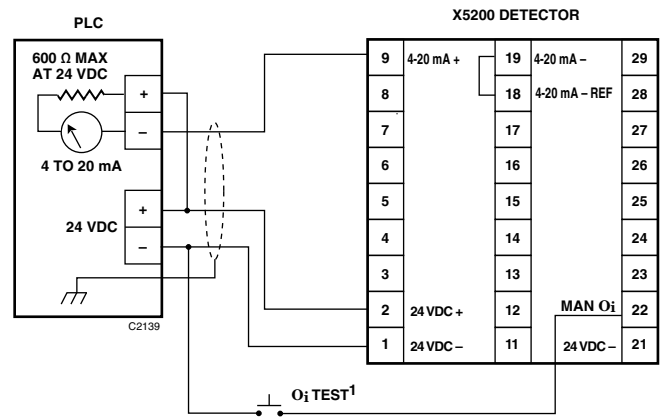
Figure 10—X5200 Detector Wired for Non-Isolated 0 to 20 mA Current Output (Sinking)
