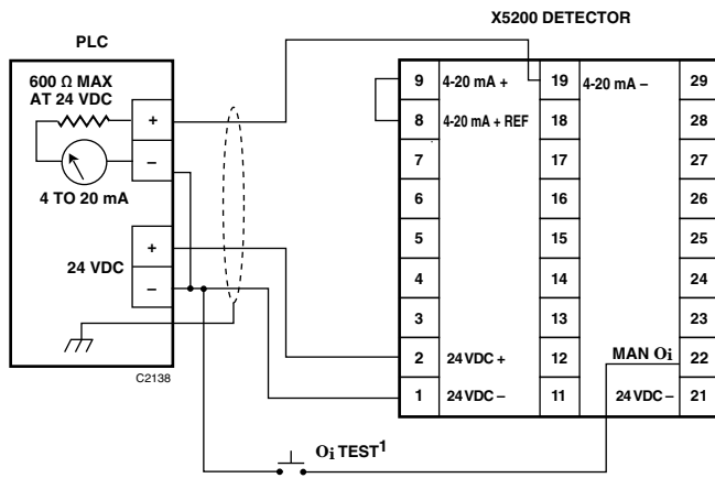
Figure 9—X5200 Detector Wired for Non-Isolated 0 to 20 mA Current Output (Sourcing)
