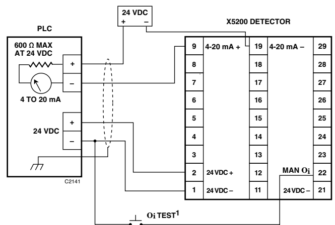
Figure 12—X5200 Detector Wired for Isolated 0 to 20 mA Current Output (Sinking)
