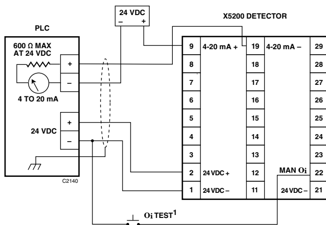
Figure 11—X5200 Detector Wired for Isolated 0 to 20 mA Current Output (Sourcing)
