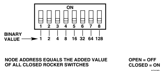
Figure 17—Address Switches for X5200
