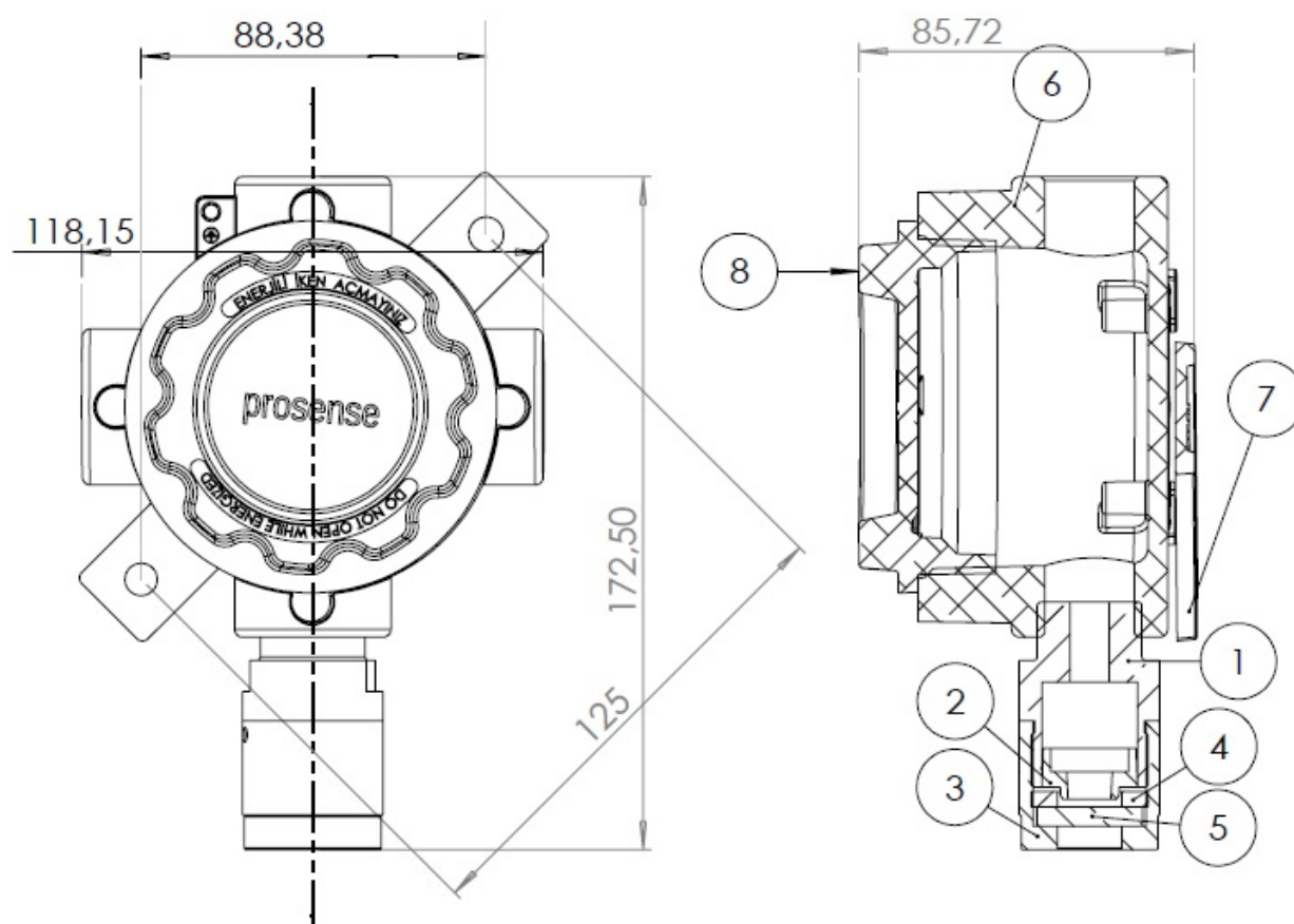
Diagram 2: Detector body size and Sensor Head components
