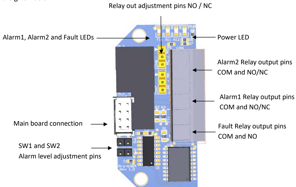
Diagram 11: Relay module
