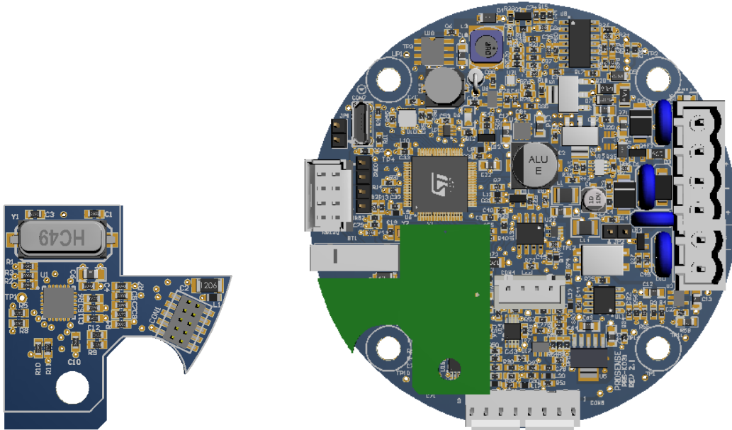
Diagram 13: HART module and mainboard with HART module
