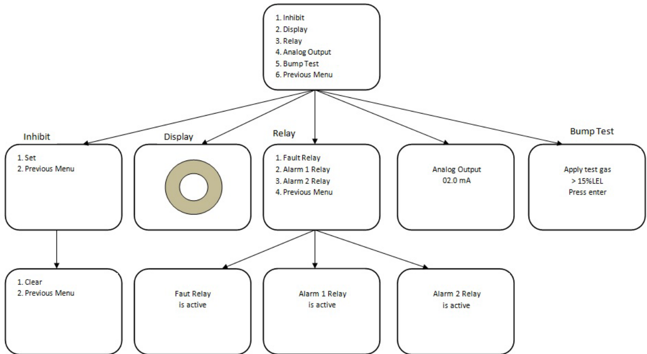
Diagram 19: Test menu structure
