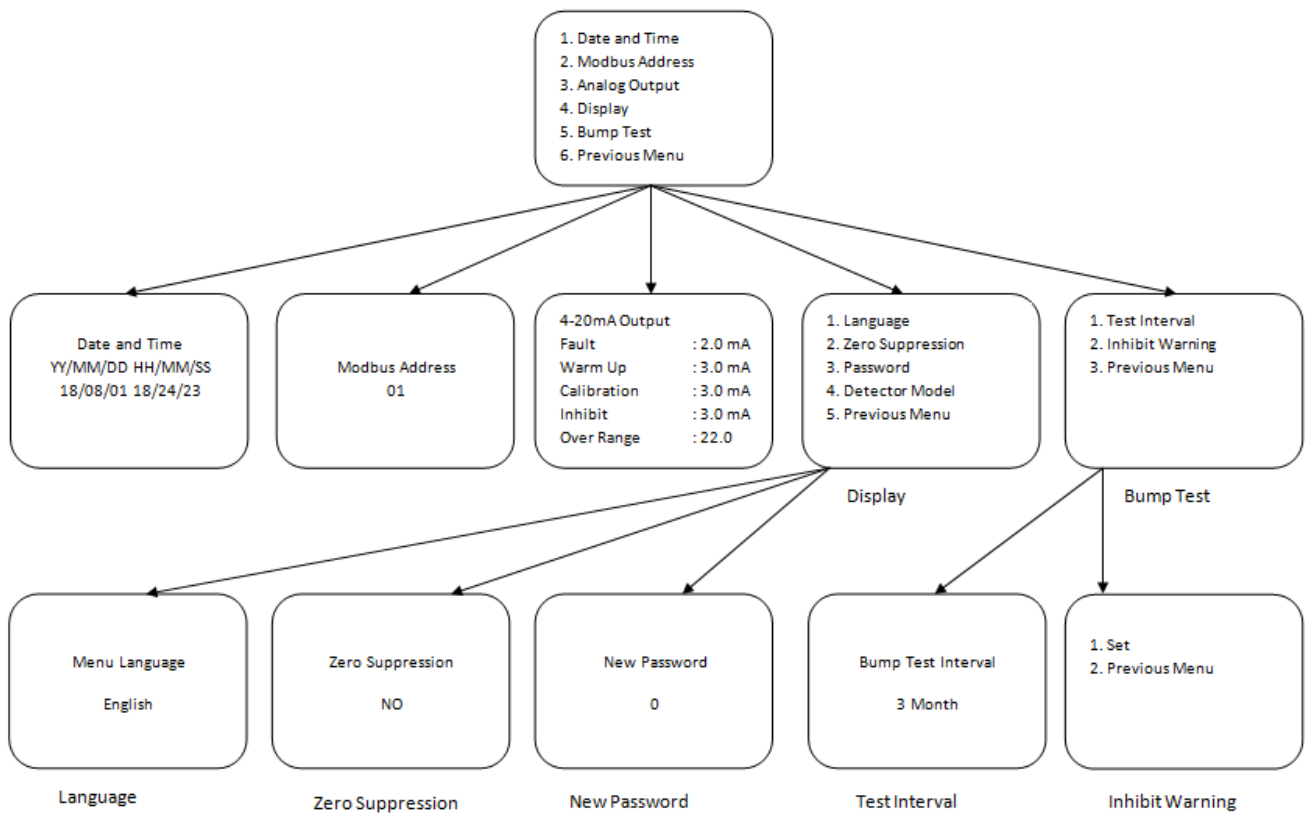
Diagram17: Configure menu structure
