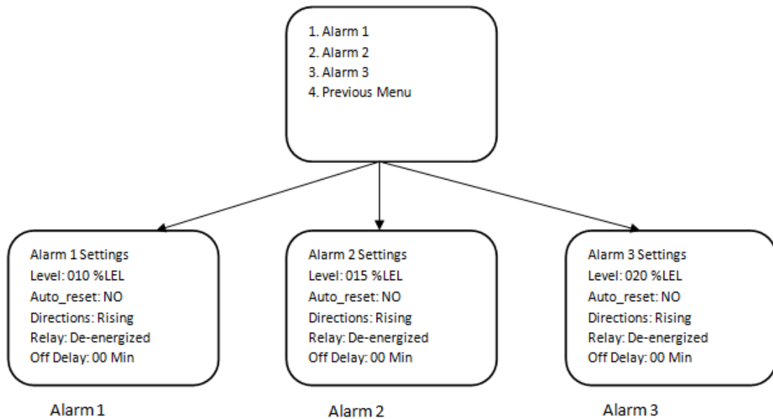
Diagram 16: Alarm menu structure
